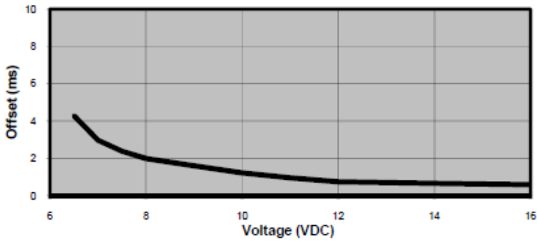
Voltage Sensitivity Summary, 6-16V
